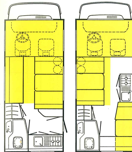
Camp 55
